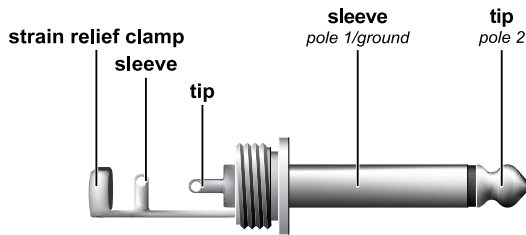
Fig. 4.1: 1/4" TS connector for foot switch
