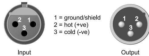
Fig. 4.2: XLR connections
