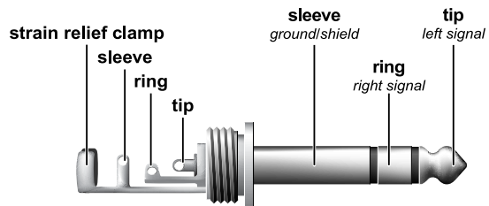
Fig. 4.5: 1/4" TRS connector for headphones
