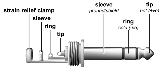
Fig. 4.4: 1/4" TRS connector
